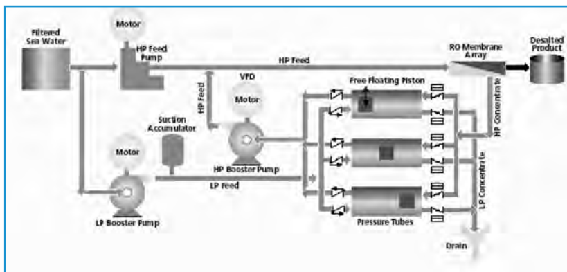
Fig 11.10 - Process flow diagram of Pressure Exchanger
